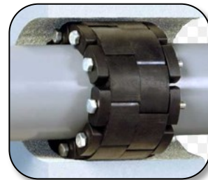
Penetration Seals
