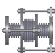
PBI Pressure Balanced In-Line
